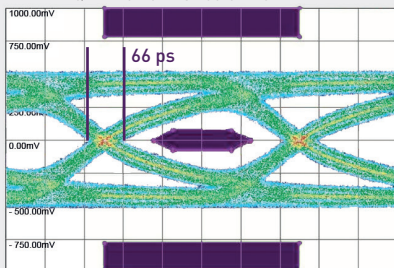
QED Performance e-Flex HDMI
